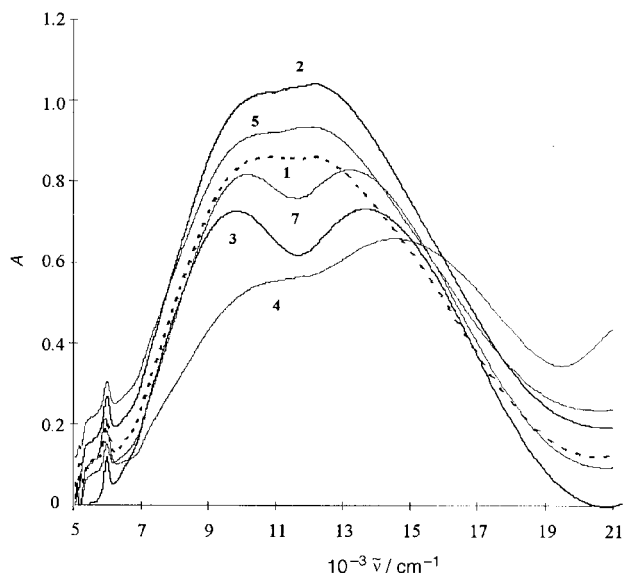
Fig. 7 Electronic reflectance spectra of some [\text{Cu}(\text{phen})_2\text{Cl}][\text{Y}] complexes
